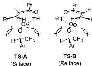
Figure 1. Template structures TS-A [( Si ) face] and TS-B [( Re ) face] for the base-catalyzed asymmetric oxygen transfer in the Weitz–Scheffer epoxidation of \alpha, \beta -enones by optically active hydroperoxides, where T^+ (either the K^+ or R_3NH^+ ion) represents the templating agent; to facilitate the discussion, the ( Si ) face and ( Re ) face descriptors for substrate 1a have been adopted for all others; actually the priorities differ only for substrate 1b
