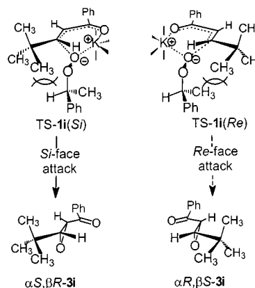
Scheme 3. Potassium-coordinated template for the enantioselective epoxidation of the tert -butyl-substituted enone 1i with the optically active hydroperoxide 2a , catalyzed by KOH
