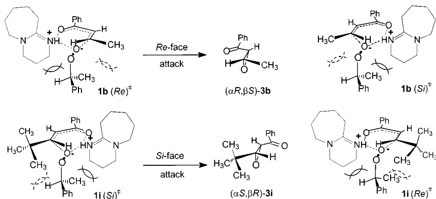
Scheme 4. Hydrogen-bonded template for the enantioselective epoxidation of the enones 1b and 1i with the optically active hydroperoxide 2a , base-catalyzed by DBU
