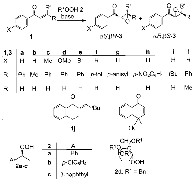
Scheme 2. Base-catalyzed enantioselective Weitz–Scheffer epoxidation of enones 1 by optically active hydroperoxides 2
